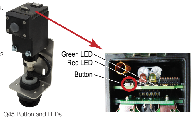
Q45 Button and LEDs
