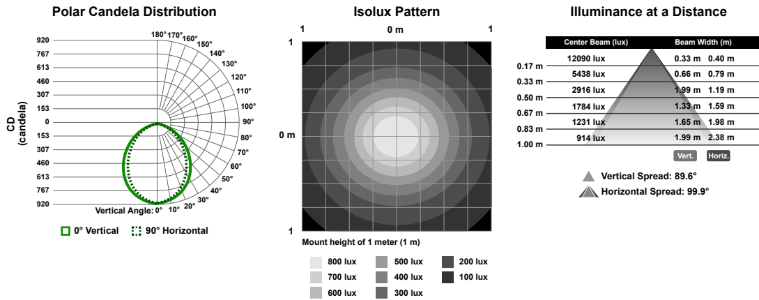
Figure 4. 900 mm Model
