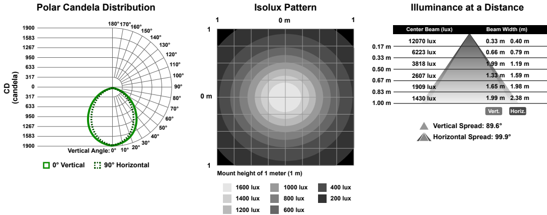
Figure 5. 1200 mm Model
