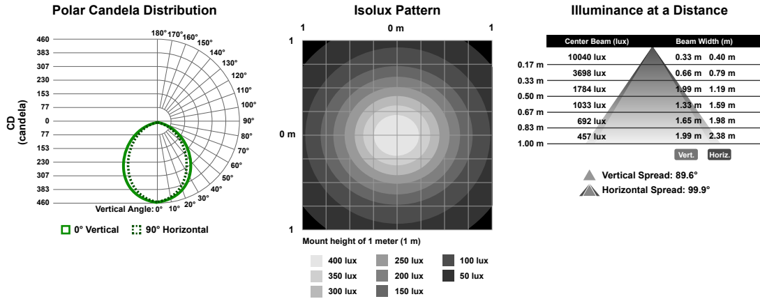
Figure 3. 600 mm Model
