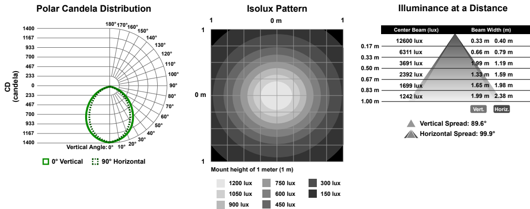
Figure 4. 900 mm Model
