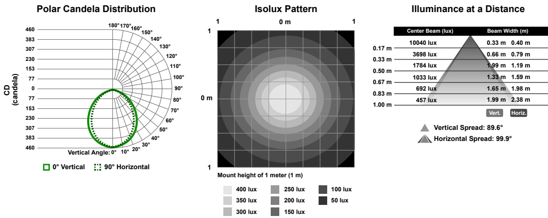
Figure 4. 600 mm Model
