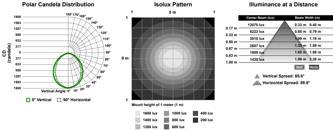
Figure 6. 1200 mm Model
