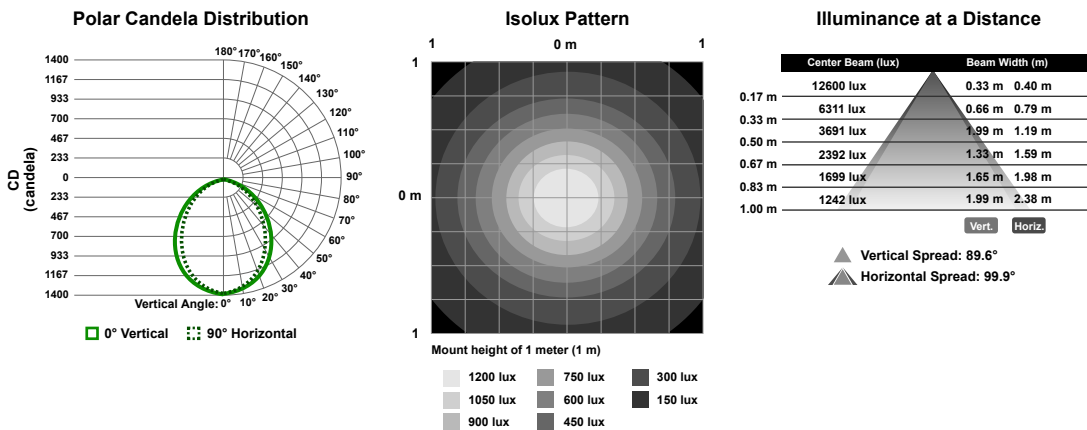
Figure 5. 900 mm Model
