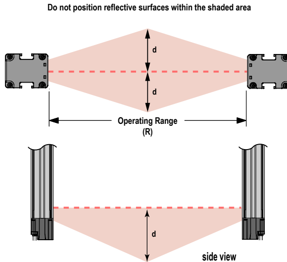
Figure 4. Adjacent Reflective Surfaces
