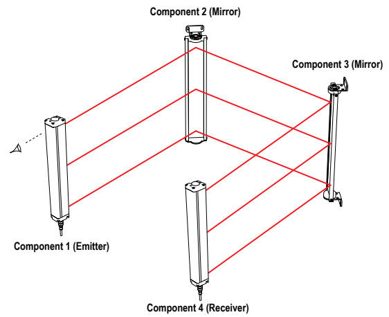
Figure 11. Corner Mirror Alignment
