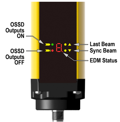
Figure 2. Status Indicators—Receiver
