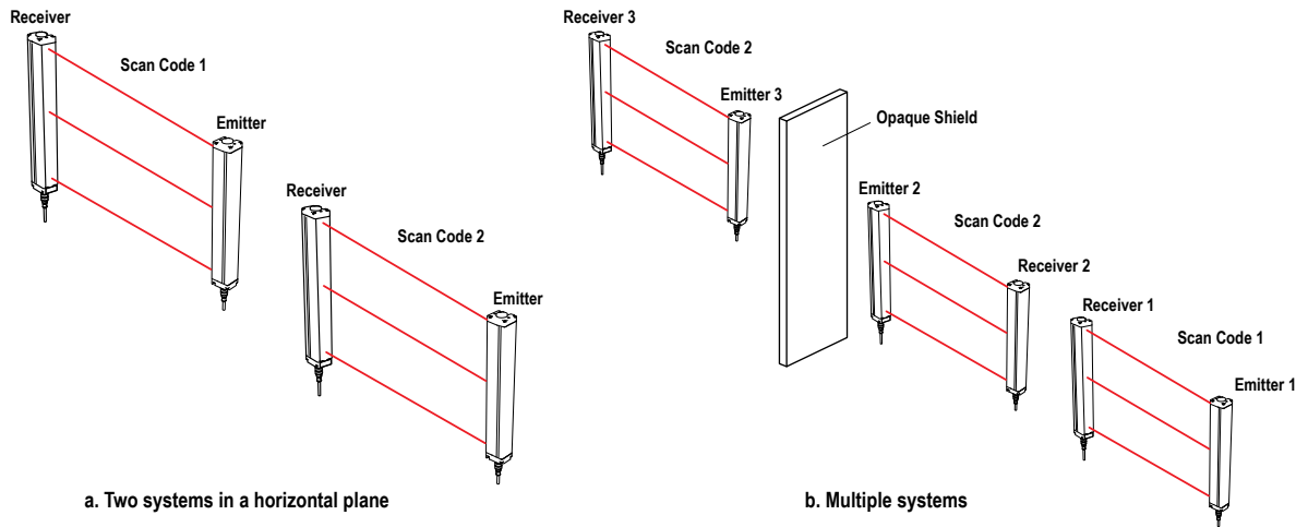
Figure 7. Installing Multiple Systems
