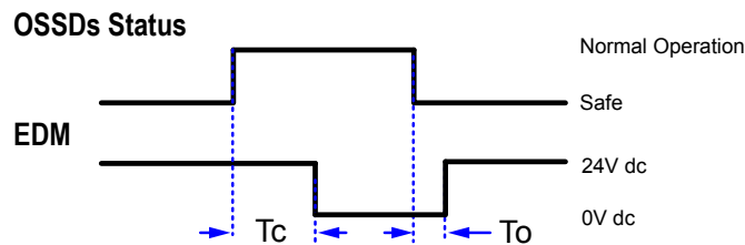
Figure 14. One-channel EDM status, with respect to safety output
