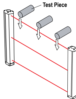
Figure 12. Trip Test
