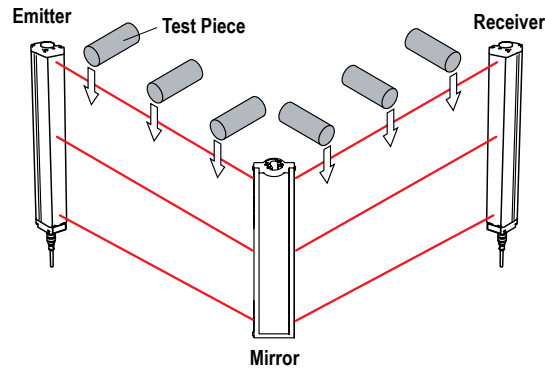
Figure 13. Trip Test with Corner Mirror
