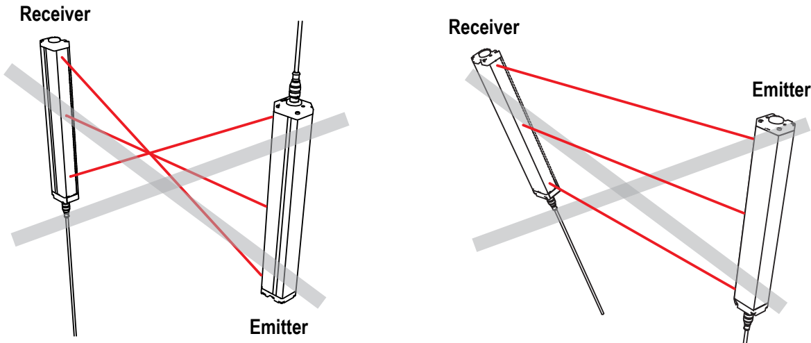
Figure 6. Examples of Incorrect Emitter/Receiver Orientation
