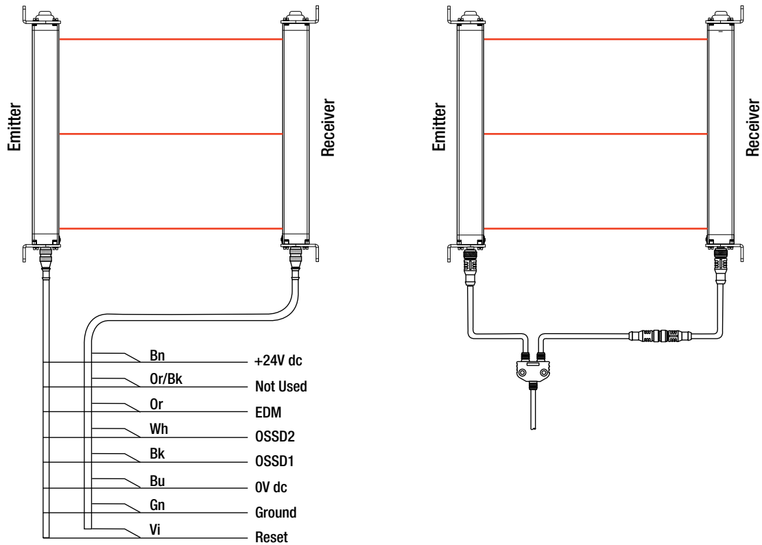
Figure 15. Individual cordsets (left) and Splitter cordsets (right)
