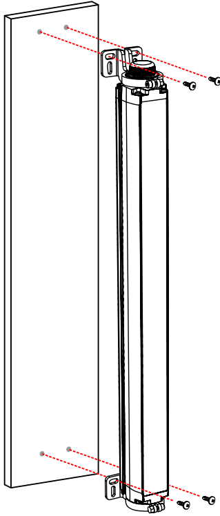
Figure 8. End-Mount Brackets
