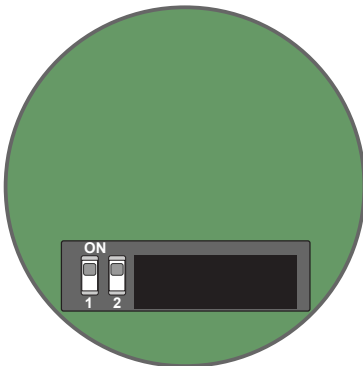
Figure 16. Emitter DIP Switches
