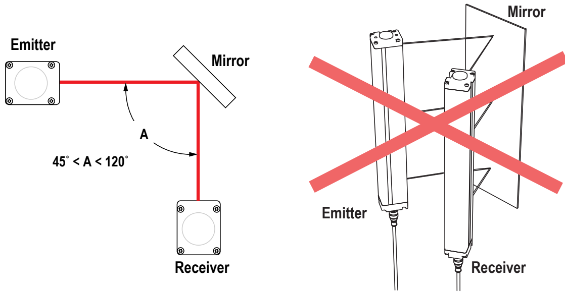
Figure 5. Using SGS sensors in a retroreflective mode
