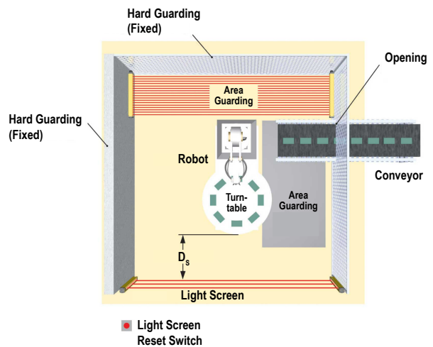
Figure 3. An example of supplemental safeguarding
