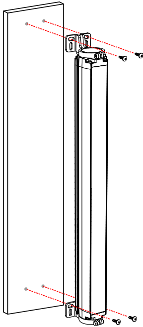
Figure 7. End-Mount Brackets
