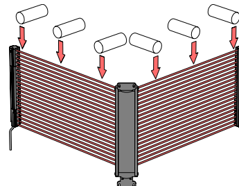
Figure 2. Trip test for corner mirror applications
