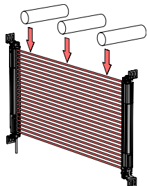
Figure 1. Trip test
