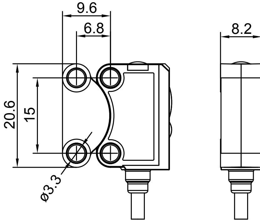
VS8 Series Sensor with SMBVS8DT Bracket
