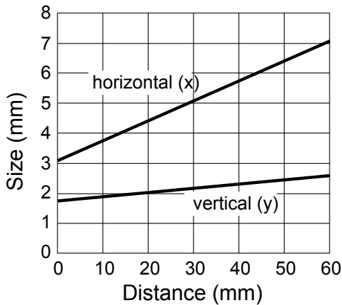
Laser Adjustable Field Background Suppression
