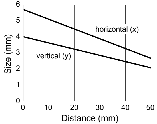
Fixed Field Background Suppression with Blue LED
