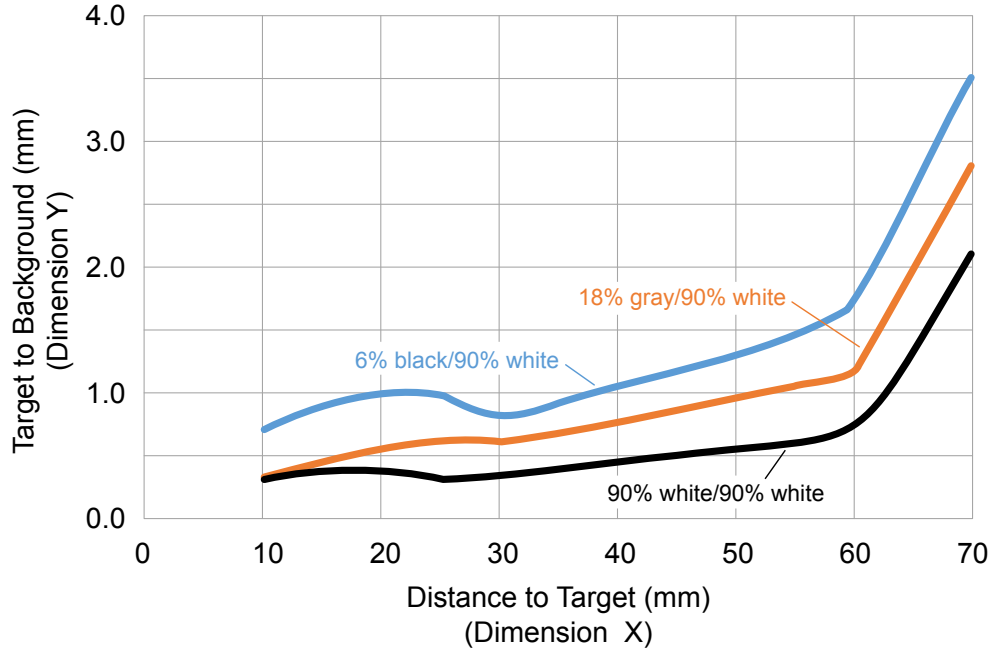
Minimum object separation for laser sensor models with background suppression
