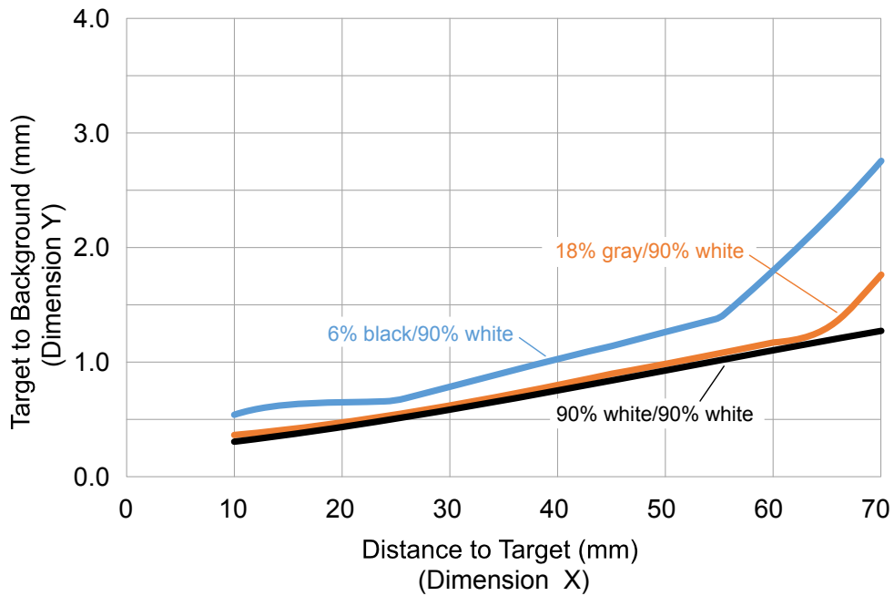
Minimum object separation for LED sensor models with background suppression
