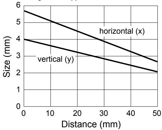
Fixed Field Background Suppression
