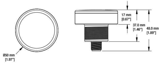
Figure 2. Quick-Disconnect Models
